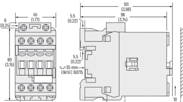
Figure 44 - 100-E26...100-E38 4-Pole Contactors with Standard Coils
