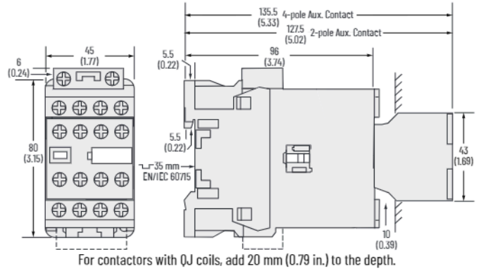
Figure 53 - 100-E26...100-E38 3-Pole Contactors with Low-consumption Coils and Side-mounted Auxiliary Contact
