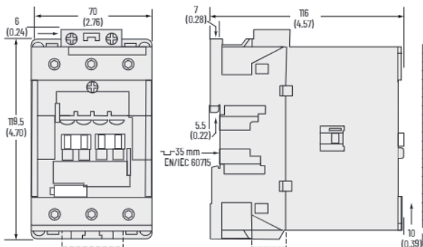
Figure 67 - 100-E80...100-E96 3-Pole Contactors with Front-mounted Auxiliary Contact
