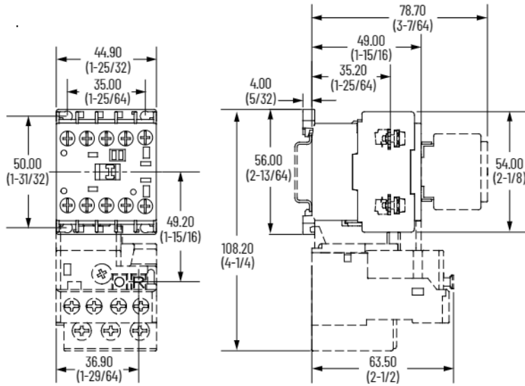
Figure 4 - Mounting Position
